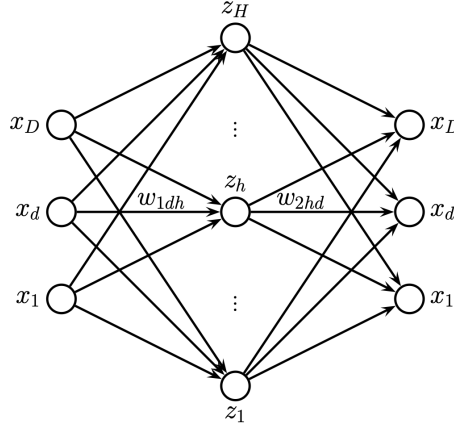
Figure 2: An autoencoder with one hidden layer MLP
